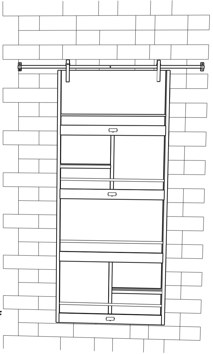
Floor guide is adjustable with the help of allen key to the bottom.
